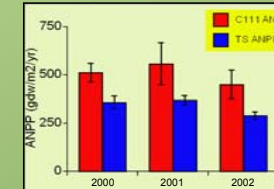
Figure 8. Annual mean ANPP for all C-111 Basin (red) and Taylor Slough (blue) sites for years in which data were available for both.
