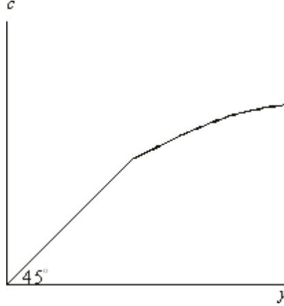
Figure 3: Adversarial, effort before – Relationship between c and y .
